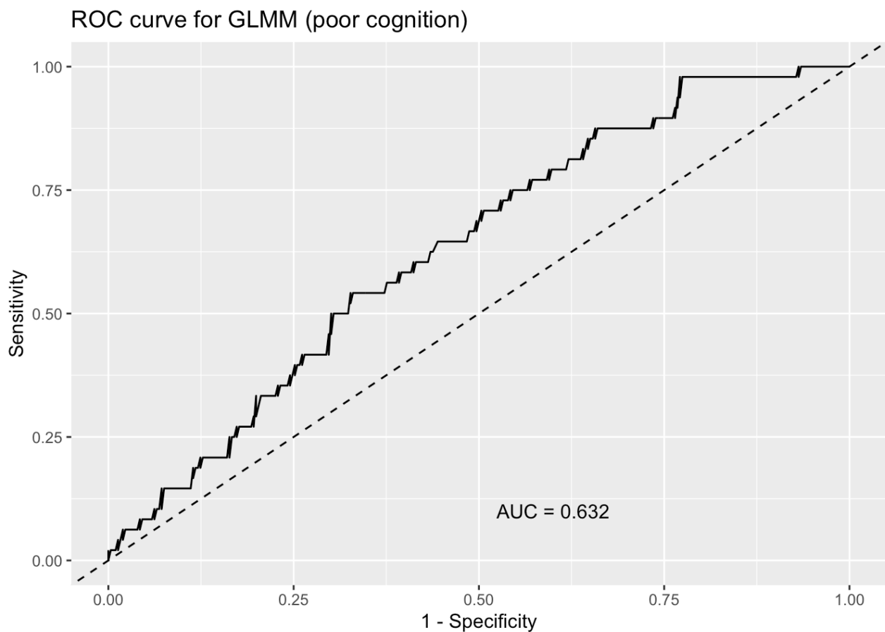
Figure 12: ROC Plot
