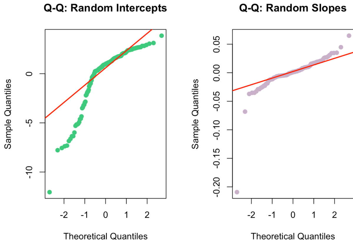
Figure 17: Random Effects Q-Q Plot
