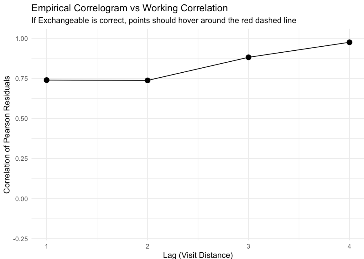
Figure 8: Empirical correlogram of Pearson residuals. The black points represent the empirical correlation at each lag, and the red dashed line represents the estimated exchangeable correlation (Math input error )
