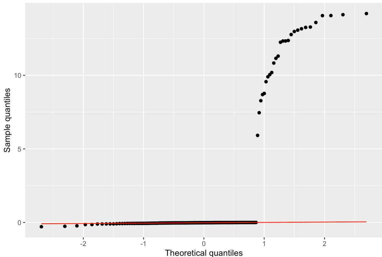
Figure 13: Q-Q plot
