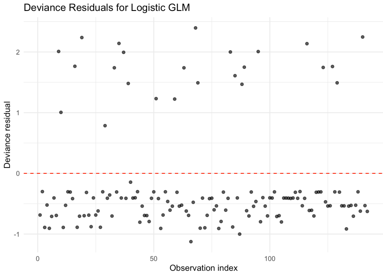
Figure 3: Deviance Residuals Plot for Logistic GLM
